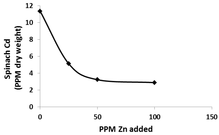
Fig. 1. Effect of ZnSO 4 amendment rate (PPM elemental Zn) to soil on spinach leaf Cd (PPM dry weight, across soils), pot experiment 1.
